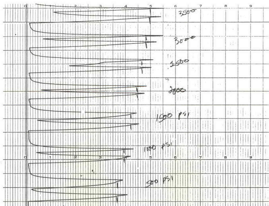
Fig. 8. --Typical Strip-chart Record of Melting for Lead (upper) and Zinc (lower).
